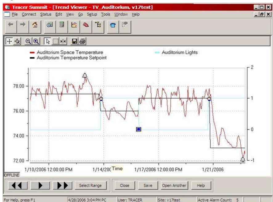
Figure 2. Trend Viewer
