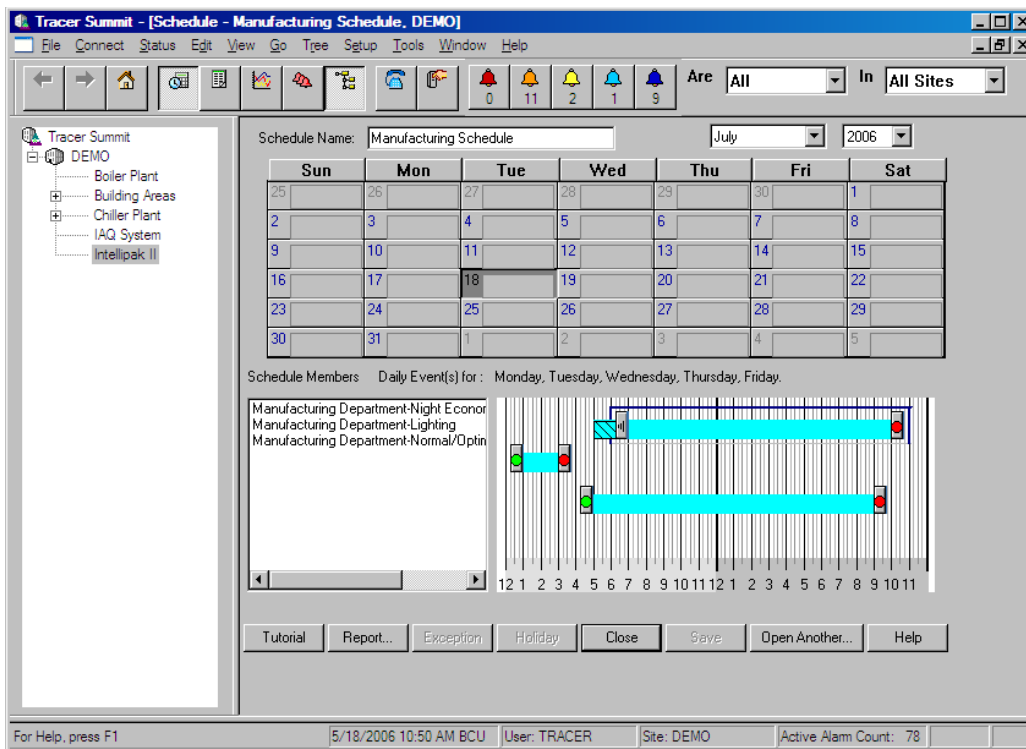
Figure 3. Scheduling editor
