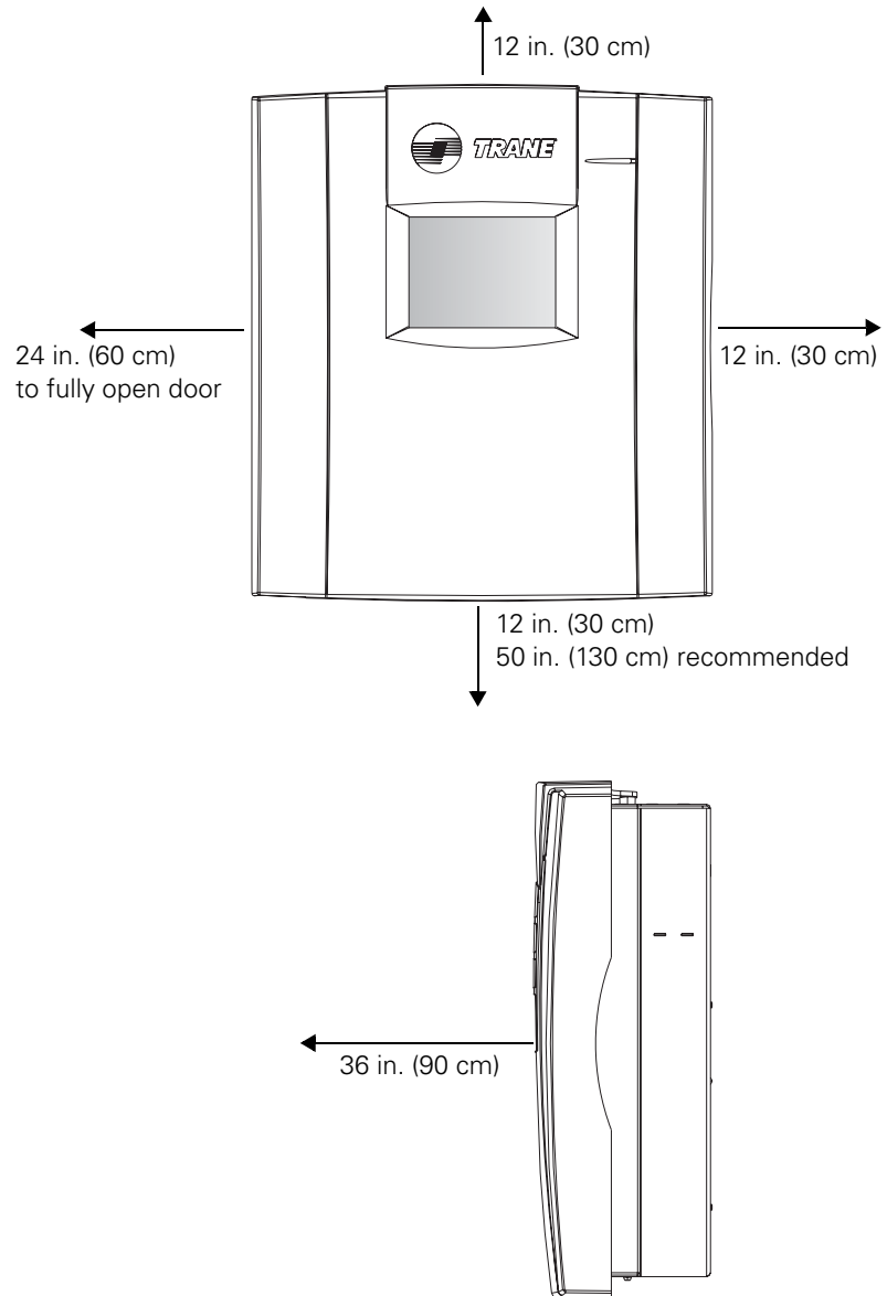
Figure 8. Minimum clearances for the BMTX BCU enclosure
