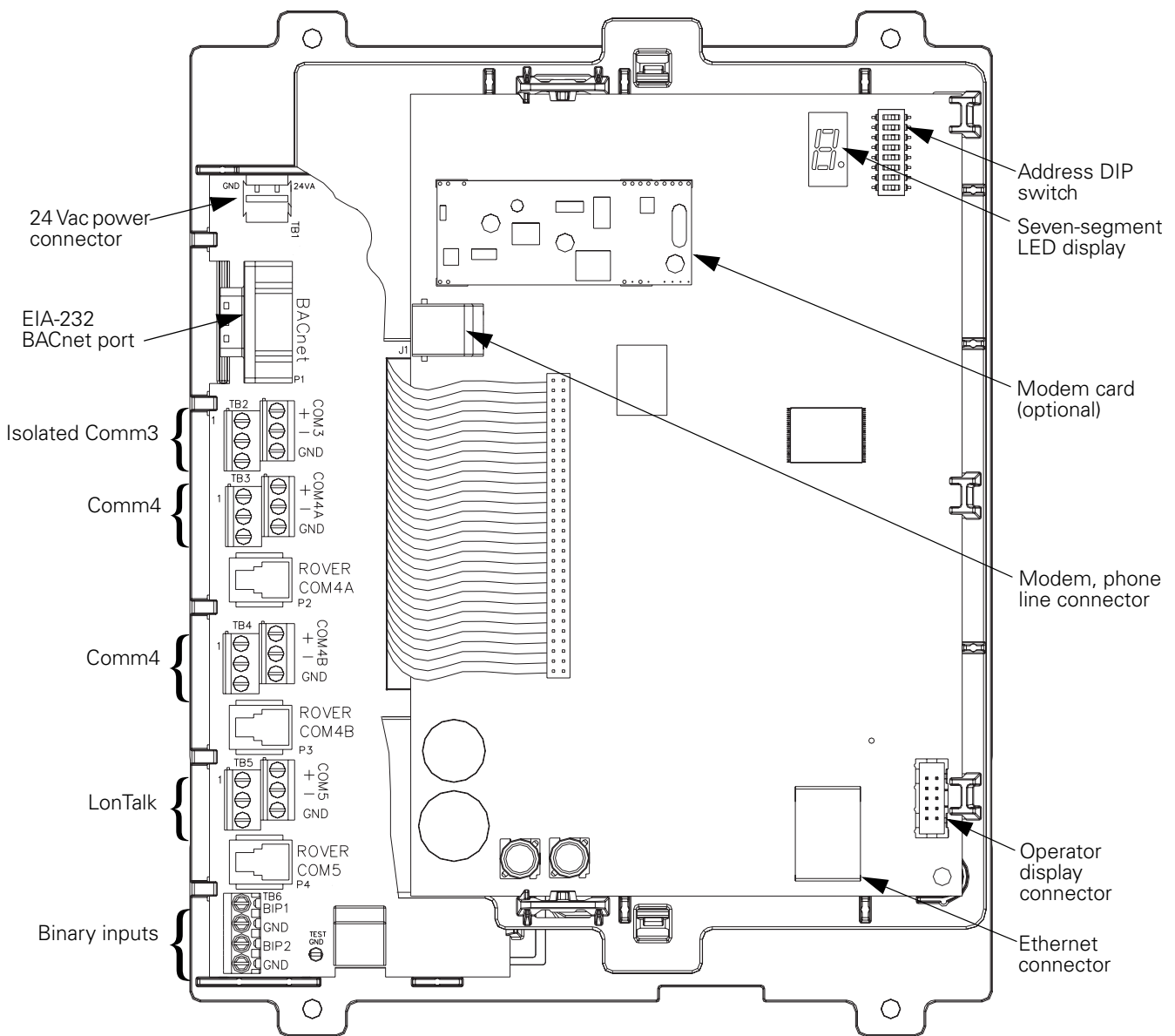
Figure 5. BMTX BCU board components
